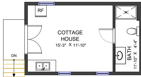
Cottage House Ceiling Height: 10'
