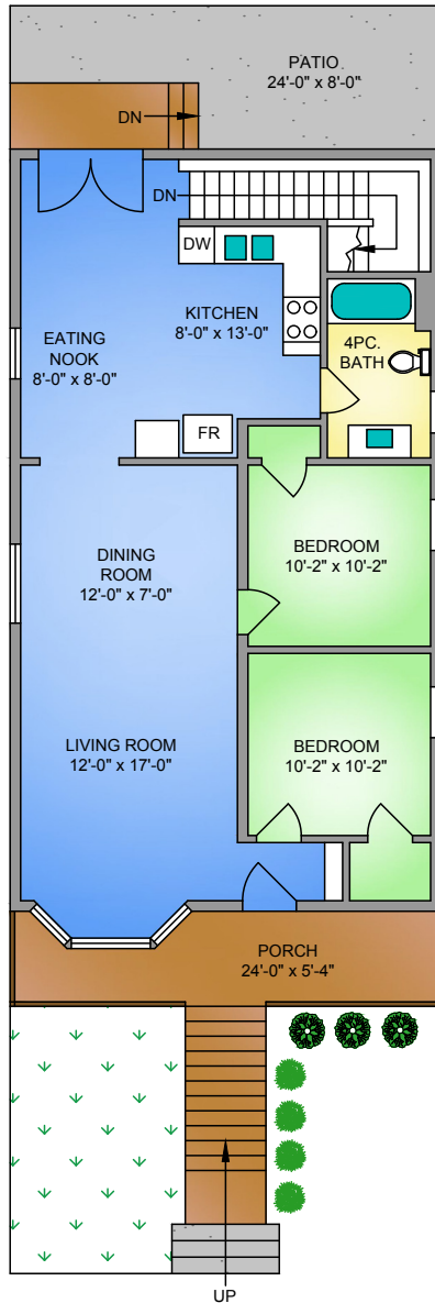
MAIN FLOOR 1040 SQ. FT. 9'-0" CEILING HEIGHT
