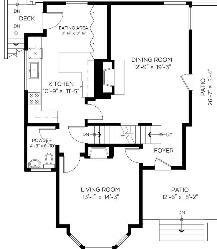
Main Floor Plan Floor Area: 884 sq.ft
