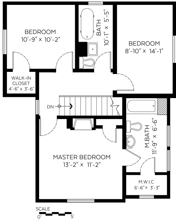
Upper Floor Plan Floor Area: 754 sq.ft
