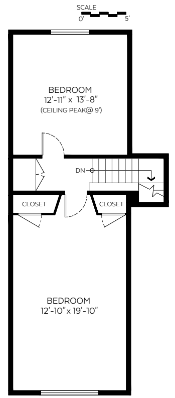
Upper Floor Plan Floor Area: 596 sq.ft. Ceiling Peak @ 9 ft.
