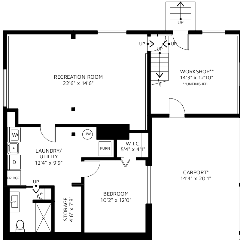
BASEMENT
