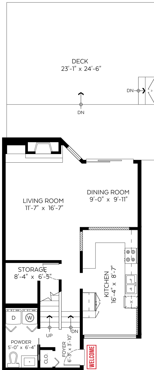
Main Floor Plan Floor Area: 700 sq.ft. Ceiling Height: 8'
