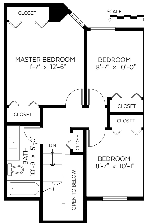
Upper Floor Plan Floor Area: 583 sq.ft. Ceiling Height: 8'
