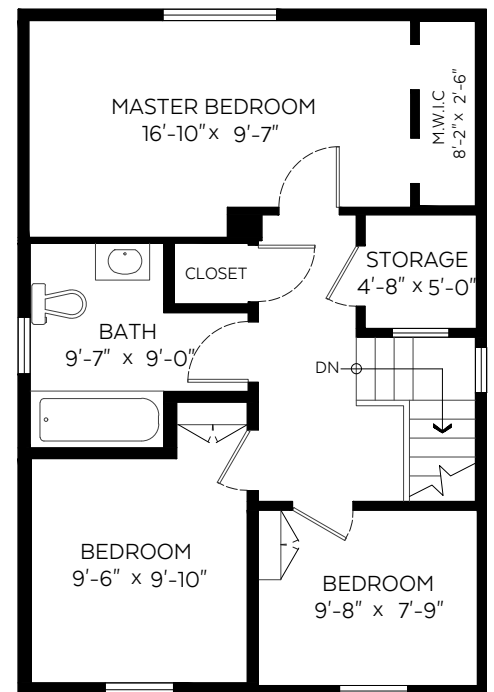
Upper Floor Plan Floor Area: 626 sq.ft.
